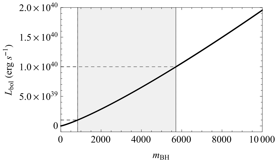
Figure 2. The curve of the bolometric luminosity as a function of BH mass for the PRCB magnetic fields at ISCO become saturated. The shaded area indicates the BH mass ranges between 839M_{\odot} and 5719M_{\odot} for the bolometric luminosity ranges from 10^{39} to 10^{40} erg s ^{-1} .
