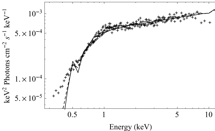
Figure 1. The simulated and observed spectra of NGC 1313 X-1 associated with the 3:2 QPOs. The solid and dashed lines represent the model spectra with a_* = 0.3 and a_* = 0.998 , respectively. The symbol “+” denotes the observed spectrum (without error bars) with data taken from Bachetti et al. (2013).
