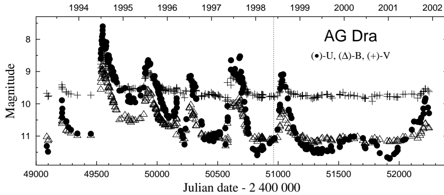
Figure 6. As in Fig. 3, but for AG Dra.
