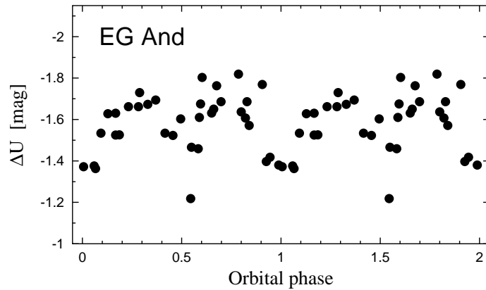
Figure 1. The LC of EG And in U . It consists of only the data published in this paper (Table 1). The data were folded with the ephemeris for the primary minima, Min = JD\ 2\ 446\ 336.7 + 482 \times E (Skopal 1997).
