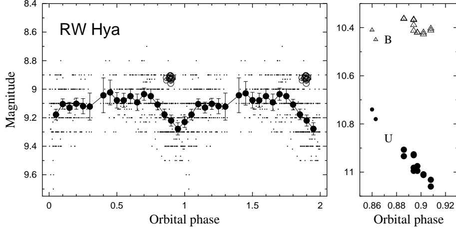
Figure 7. Left: Phase diagram for our visual estimates of RW Hya: (dots) - all individual observations, (●) - mean values made in bins of \Delta\varphi = 0.05 with corresponding uncertainty (rms). The average uncertainty of the individual estimates was adopted to 0.3 mag. Our photoelectric V measurements (○) and those of Munari et al. (1992) (◦) are compared. The difference between the visual and photoelectric data sets is probably caused by the different comparison stars used. Right: Detail of a phase diagram for our photoelectric measurements in U and B . The smaller marks denote the data of Munari et al. (1992).
