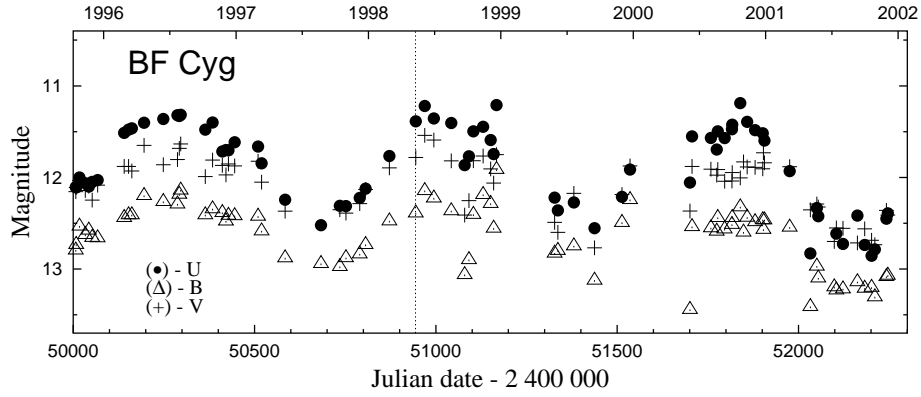
Figure 3. The UBV LCs of BF Cyg. New data presented in this paper are plotted on the right of the vertical dotted line.
