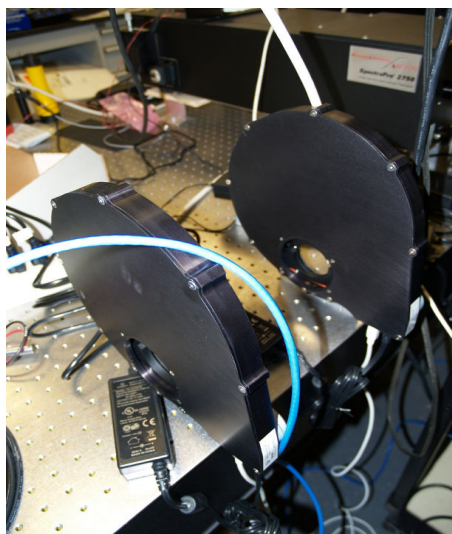
Figure 1. The filters wheels with narrow band filters and polarization optics tested at the National Center for Atmospheric Research, Boulder, USA.
