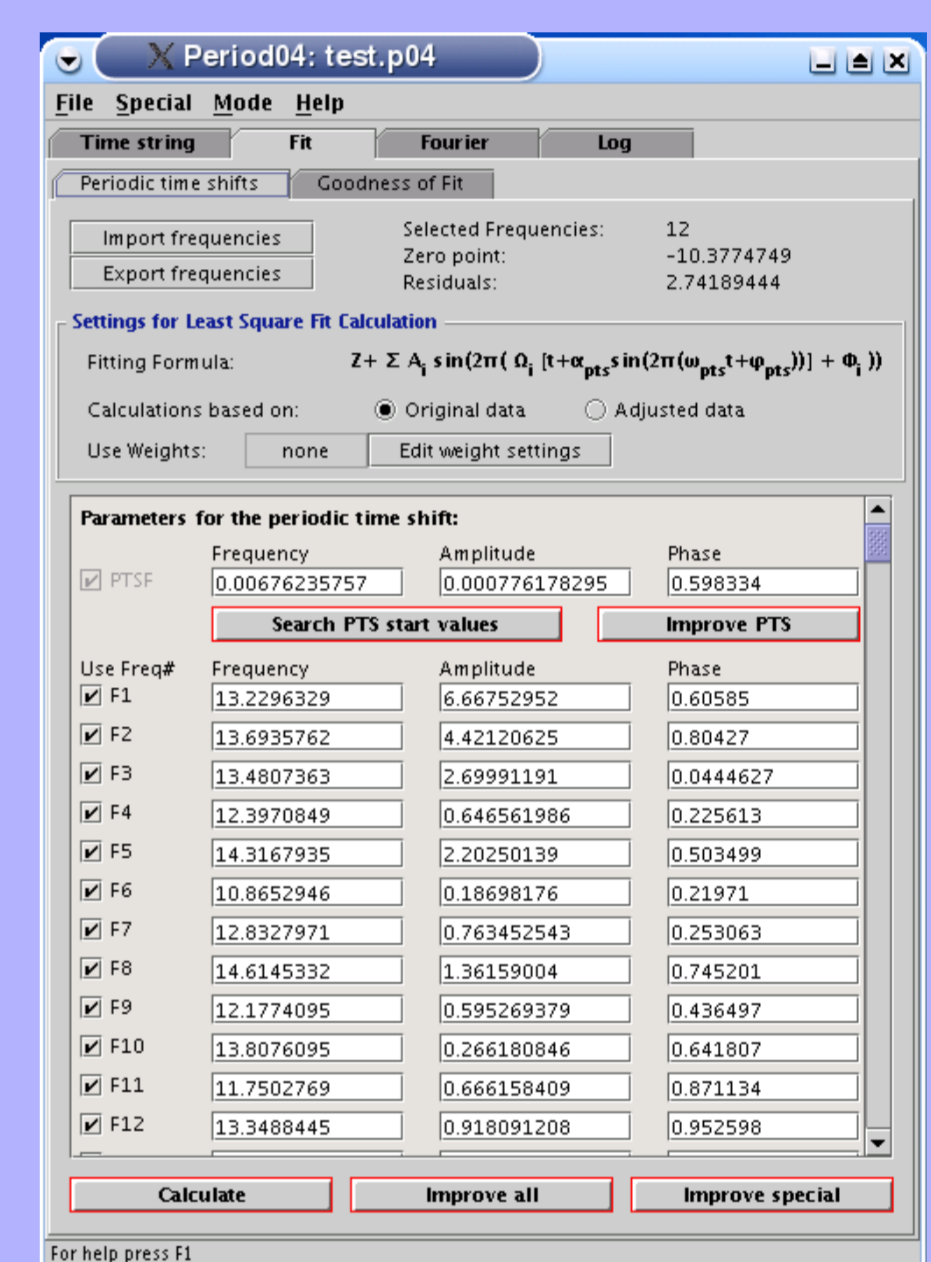
Fig. 2: The periodic time shift calculation mode
