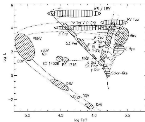
Figure 1. The H-R diagram showing the location of various types of pulsating variables (Jeffery, 2008). Some more types are listed in Table 1.
