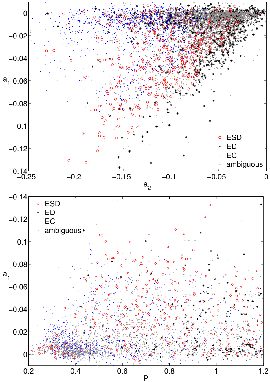
Figure 4. Dependences between coefficients a_1 - a_2 and a_1 - P , where P is the orbital period.
