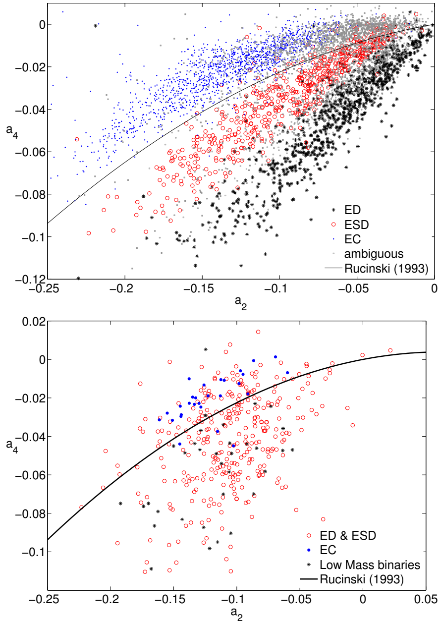
Figure 3. The relationship between Fourier coefficients a_2 and a_4 and comparison of this relationship with the data from the NSVS database. The solid line represents the border separating contact systems from semi-detached and detached ones (Rucinski, 1993). The grey squares represent systems with an ambiguous classification from the ACVS catalogue.
