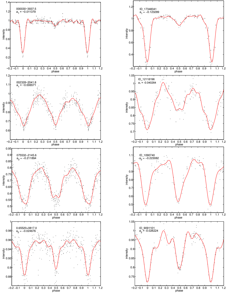
Figure 2. The light curves from the ASAS and NSVS databases focus on the difference between depths of primary and secondary minima represented by the Fourier coefficient a_1 (top two rows). The smaller value of this coefficient, the greater difference between depths of primary and secondary minima. The light curves from the ASAS and NSVS databases focus on the amplitude of the light curve changes represented by the Fourier coefficient a_2 (last two rows). The smaller the value of this coefficient, the greater the amplitude of the light curve changes.
