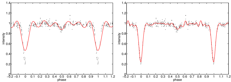
Figure 1. Comparison of two decompositions in the presented light curve (the system with catalogue ID 000030-3937.5 from the ASAS database). Left: the fit where we used the Fourier polynomial of the 6 th degree. Right: the 20 th degree of a polynomial is used.
