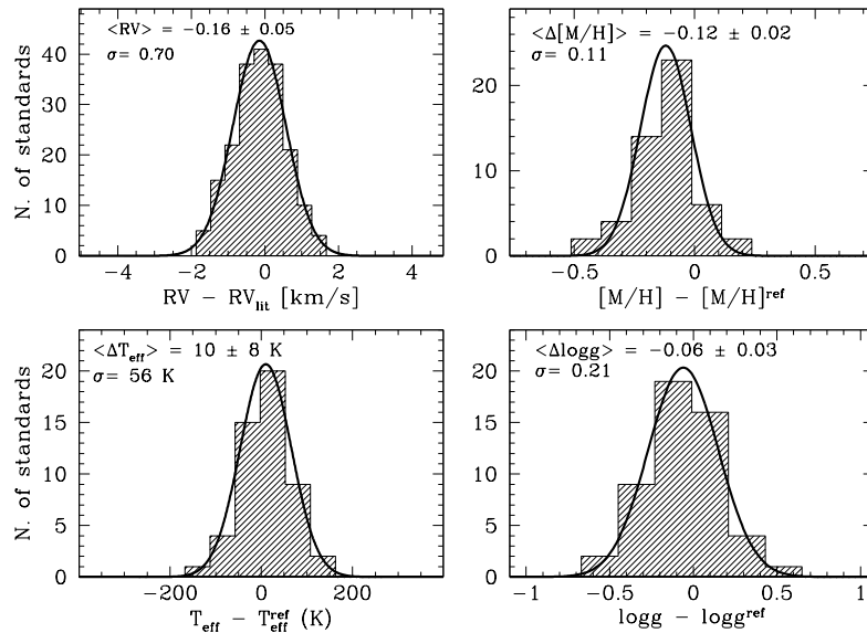
Figure 1. Distribution of shifts in RV for 215 measurements of IAU standards and in atmospheric parameters ( T_{\text{eff}} , \log g , [M/H] ) for 50 template RC stars from literature.
