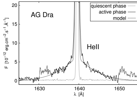
Figure 1. Broadening of the HeII 1640Å line wings by Thomson scattering in symbiotic star AG Dra during an active phase (Sekeráš & Skopal, 2012).
