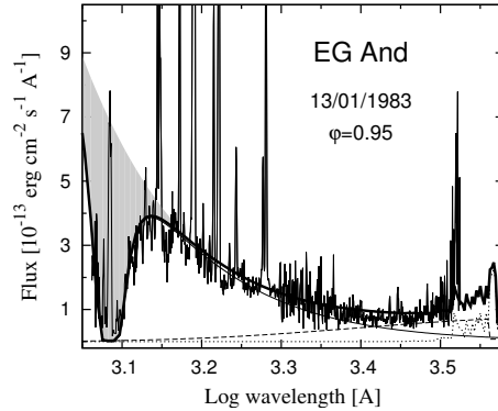
Figure 3. Attenuation of the continuum in the spectrum of symbiotic star EG And by the Rayleigh scattering (gray area, Skopal, 2005).
