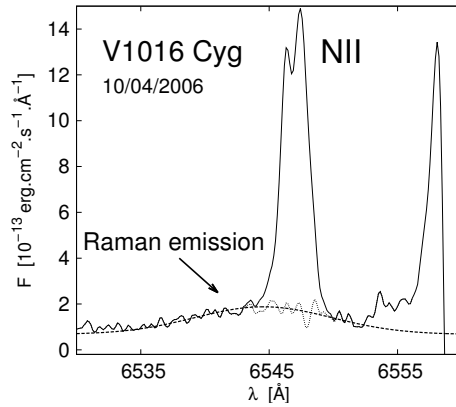
Figure 2. Raman emission in the spectrum of symbiotic star V1016 Cyg (Sekeráš & Skopal, in preparation).
