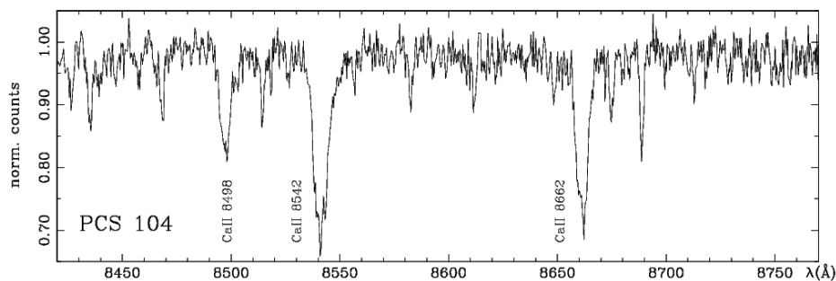
Figure 1. RAVE spectrum of the PCS 104 object collected on July 7, 2006. Lines of the Ca II triplet are identified.
