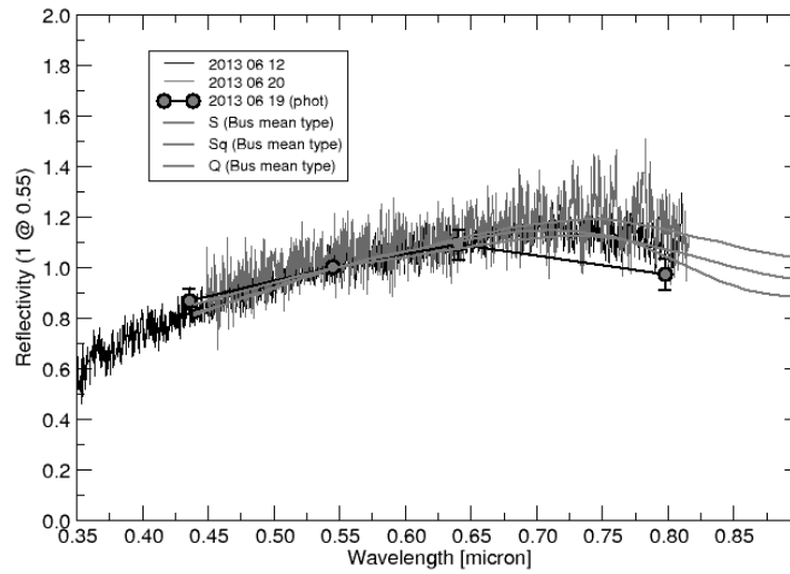
Figure 4. B&C spectra of asteroid 2002 GT. Averaged spectra relative to the S, Q and Sq types confirm that the Sq type best fits the observations.
