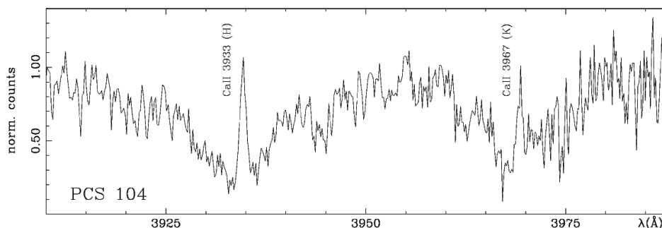
Figure 2. ECHELLE spectrum of the PCS 104 object collected on May 10, 2012 centered on the H&K Ca II doublet. Narrow emission lines superimposed on the larger absorptions are indicative of chromospheric spot activity.
