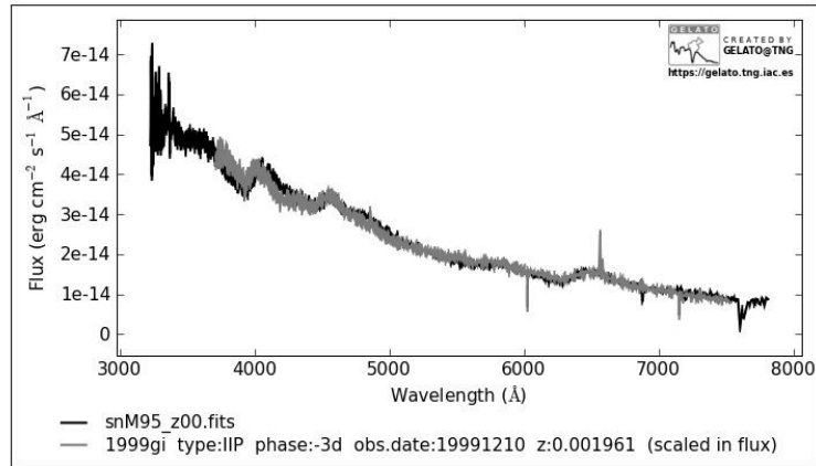
Figure 3. 1.22m + B&C spectrum of the SN 2012aw in M95 collected on Mar 19, 2012 and overplotted the 1999gi type-IIP.
