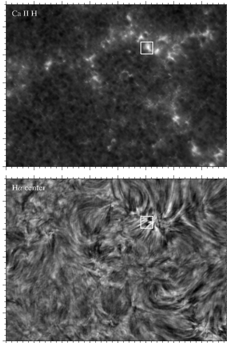
Figure 1. Images of the quiet-Sun network recorded by DOT on 19 October 2005. Top: the temporal mean of the Ca II H image sequence over its 71-min duration. Bottom: the H \alpha image taken at 10:36:21 UT in the line center at the moment of the best seeing occurred in the 41 st min after the start of the observation at 09:55:20 UT. The square defines the network element selected for this study and displayed in detail in Figs. 4–7. Field of view: 79 \times 58 arcsec 2 . Tickmark spacing: 2 arcsec.
