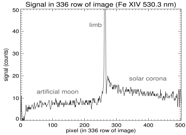
Figure 8. Plot of the signal taken from row 336 (perpendicular to the solar limb) of the narrow-band image of the corona shown in Fig. 6. Individual pixels covering the artificial moon, solar limb and the solar corona are shown.
