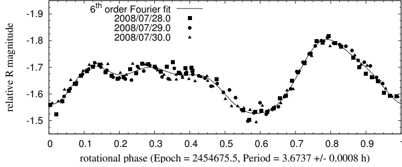
Figure 3. The composite lightcurve of asteroid Astapovich between July 28–30, 2008.
