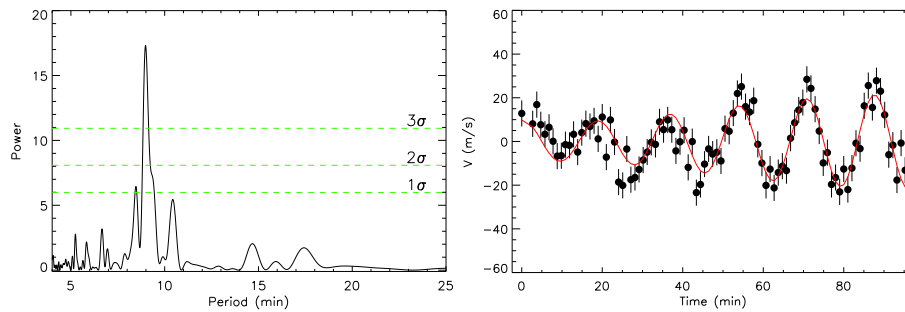
Figure 1. Left panel: Periodogram showing discovery of 9-min pulsational signal in the combined RVs of 29 Nd III lines in HD 75445. Right panel: Mean RV variation of 40 Ce II lines in \beta CrB. Multiperiodic character of oscillation is clearly evident.
