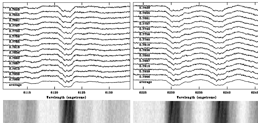
Figure 1. Spectral profile variability of the Mn II 6122 Å, Fe I 6231 Å, and Fe II 6238 Å lines in the UVES spectra of HD 21190. Spectra are labelled with Julian dates (e.g. HJD 2454047). The average spectra are plotted in the bottom of each panel. The two-dimensional images present, for the same spectral regions, the 14 observed spectra stacked. Three moving peaks are clearly visible in the cores of all presented spectral lines.
