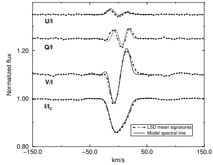
Figure 3. Tests of LSD using synthetic spectra: LSD mean signatures are extracted from a synthetic spectrum, and then compared for fidelity with the spectrum. Here, LSD mean signatures are compared with a synthetic spectral line with identical mean parameters. The amplitudes and shapes of the circular and linear polarization profiles are extremely well reproduced.
