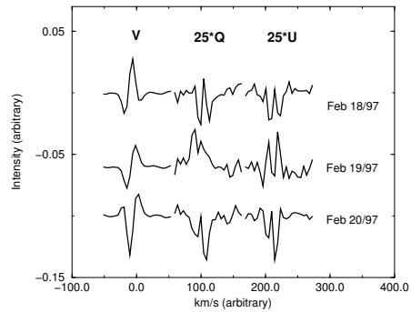
Figure 4. LSD Stokes V, Q and U mean signatures for the Ap star 78 Vir, observed on successive nights in Feb. 1997. For clarity the linear polarization profiles have been magnified by 25 \times , although they are clearly detected above the noise.
