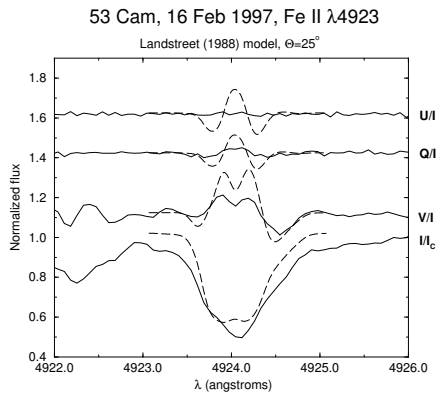
Figure 2. Solid curves (bottom to top) – Stokes I, V, Q and U profiles of Fe II \lambda 4923.9 for the Ap star 53 Cam, observed on 16 February 1997. Broken curves – Predictions of Landstreet's (1988) model. The amplitudes of all polarizations are severely overestimated by the model (by a factor of 2 for Stokes V, by a factor of 4.3 for Stokes Q, and by at least a factor of 8.3 for Stokes U).
