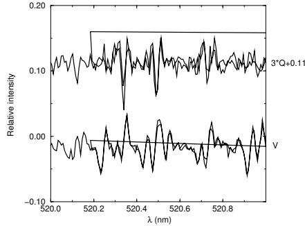
Figure 1. Stokes V (bottom) and Q (top) spectra of \beta CrB, obtained using the MuSiCoS spectropolarimeter. Each spectrum shows two overlapping échelle orders. Both V and Q are clearly detected above the noise level.
