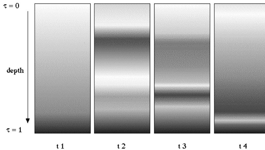
Figure 2. This is a mental picture of what kind of stratification process could occur in the photosphere of an Ap star (see text). Gray level is darker when the particle density of the considered element is higher.
