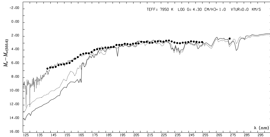
Figure 3. The ultraviolet energy distributions (in mag, relative to 5556 Å) from both ATLAS9 (full line) and ATLAS12 (dotted line) models are compared with the IUE (dashed line) and TD1 S2/68 (dark points) observations
