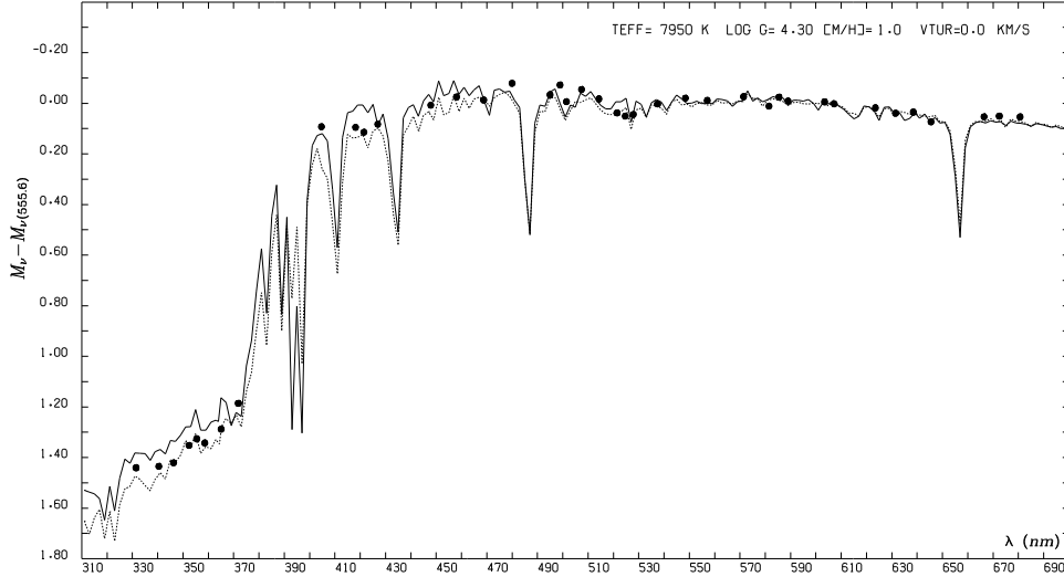
Figure 2. The visible energy distributions (in mag, relative to 5556 Å) from both ATLAS9 (full line) and ATLAS12 (dotted line) models are compared with the observations (dark points).
